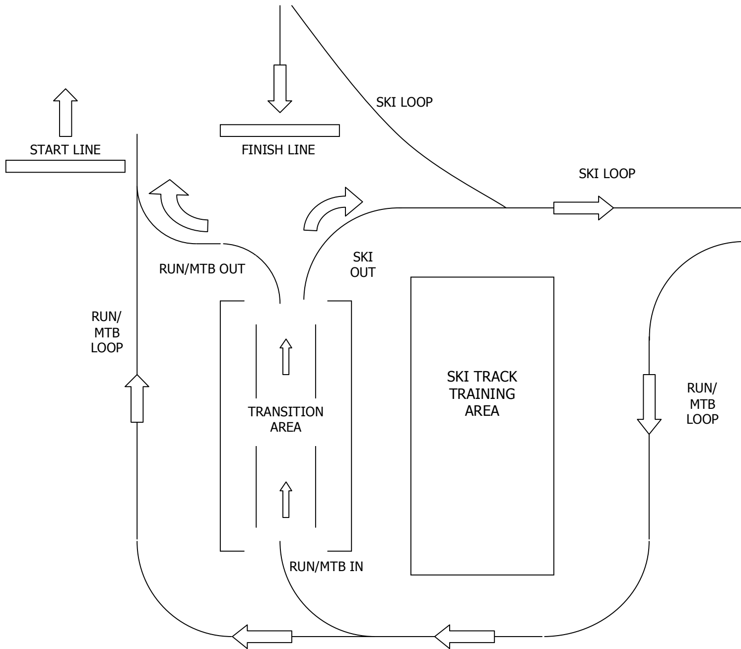
TRANSITION AREA LAYOUT
